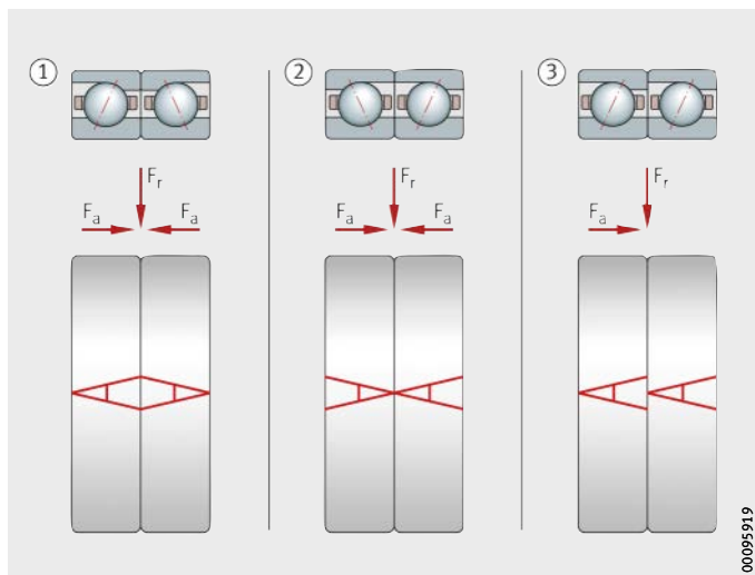
Figure 3 Bearing arrangements of a DU set
