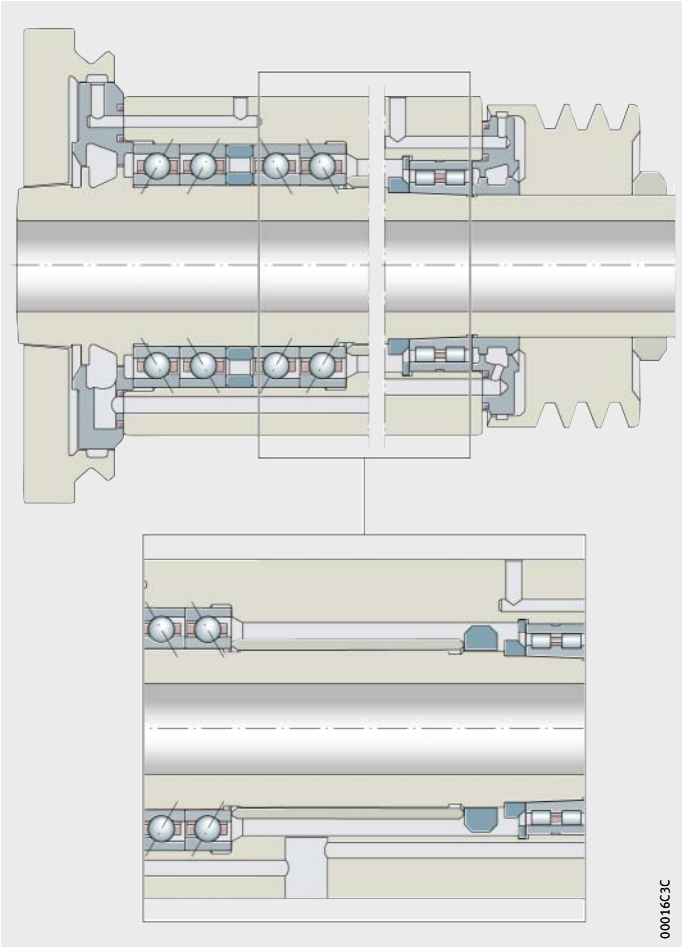
Figure 14 Grinding spindle
