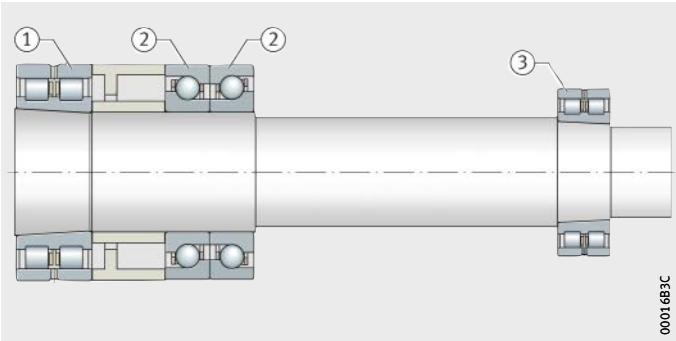
Figure 7 Bearing arrangement with axial bearings BAX
