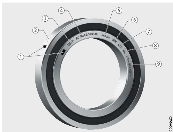
Figure 10 Marking of sealed spindle bearings
