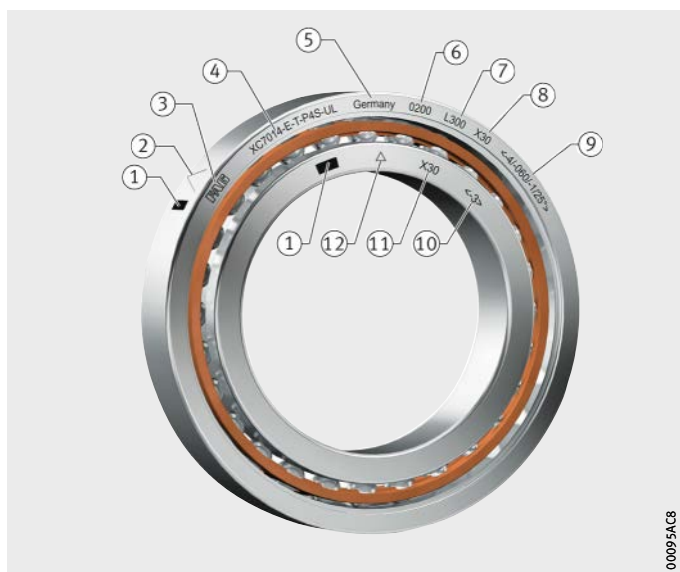
Figure 9 Marking of open spindle bearings
