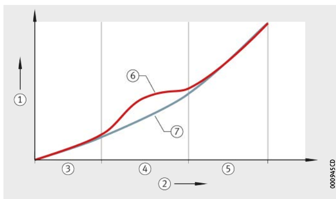
Figure 4 Speed/temperature behaviour of cylindrical roller bearings with cage guided on outer ring with oil lubrication
